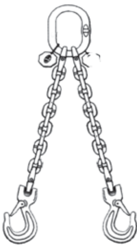
Clevis Hook with Regular Latch
